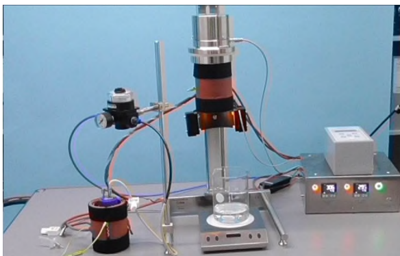
Fig 1: VARBasic2Go Unit with thermal option.
